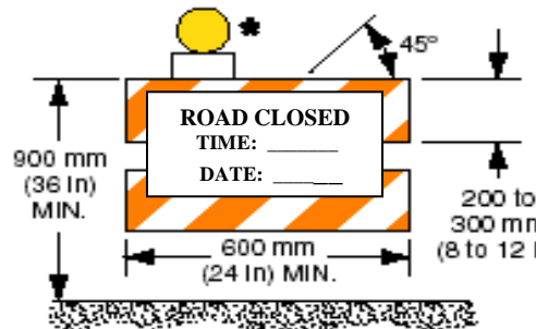
Type I or Type II barricade
