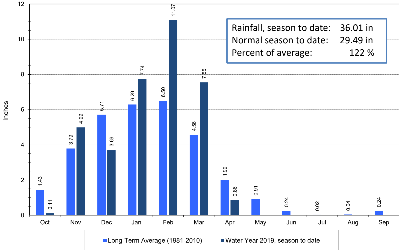
Figure 1. Monthly Rainfall, City of Santa Cruz, 04/017/2019
